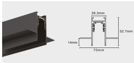
TLS-ECO-MR2X0(A) (X:1/ 2 / 3M)
