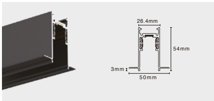
TLS-ECO-MR2X0 (X:1/ 2 / 3M)
