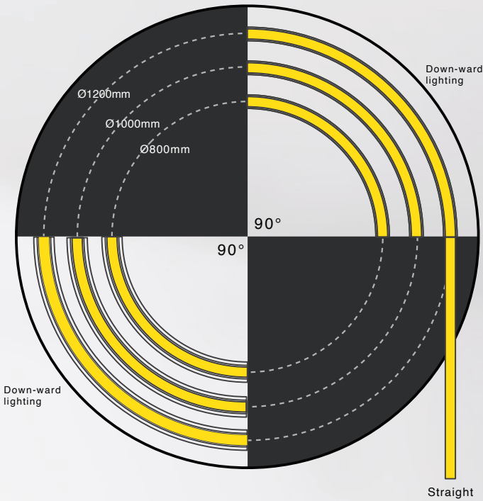
Trimless track (12.5mm/9.5mm)
